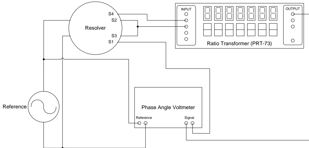
Figure 1 – Resolver Test Setup
